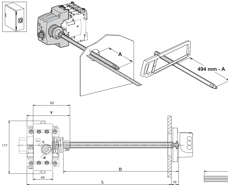
Rotary handle: side mounted control
